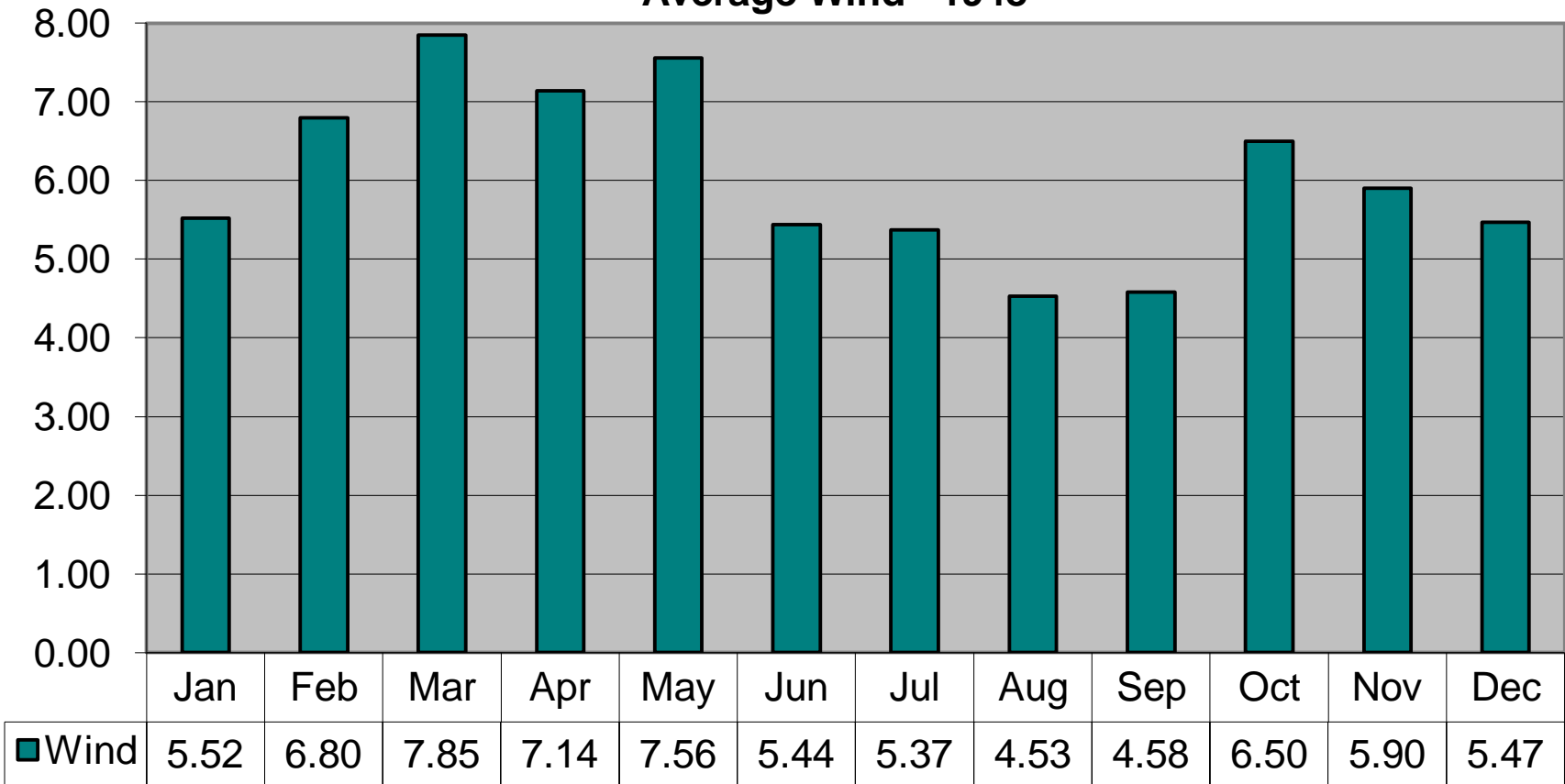
Average Wind - 1948
