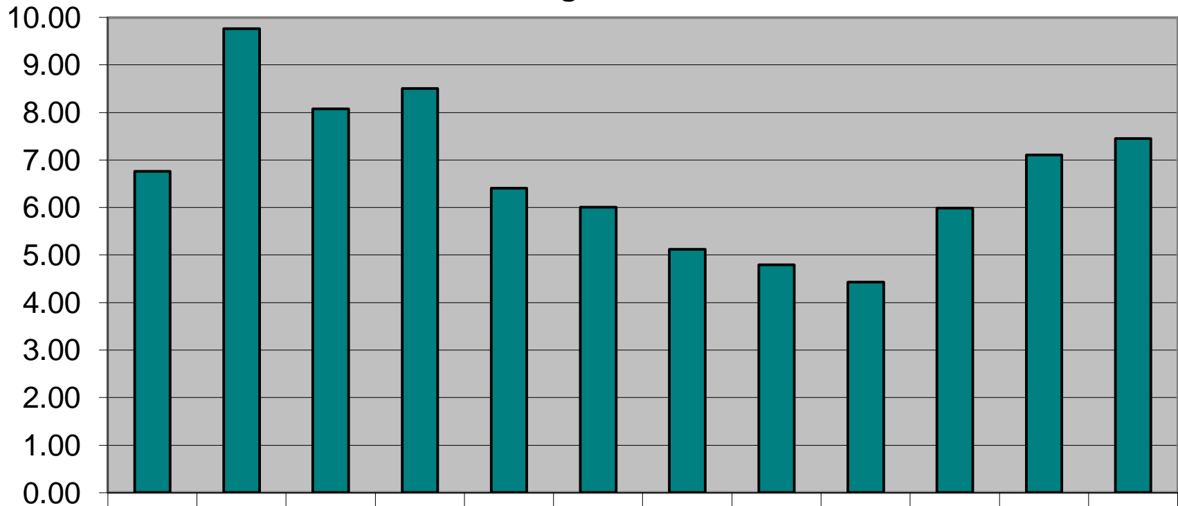
Average Wind - 1947
