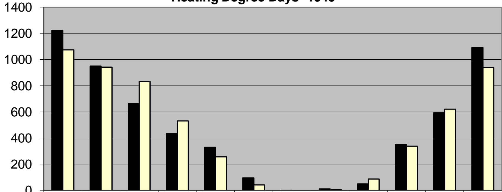
Heating Degree Days -1945
