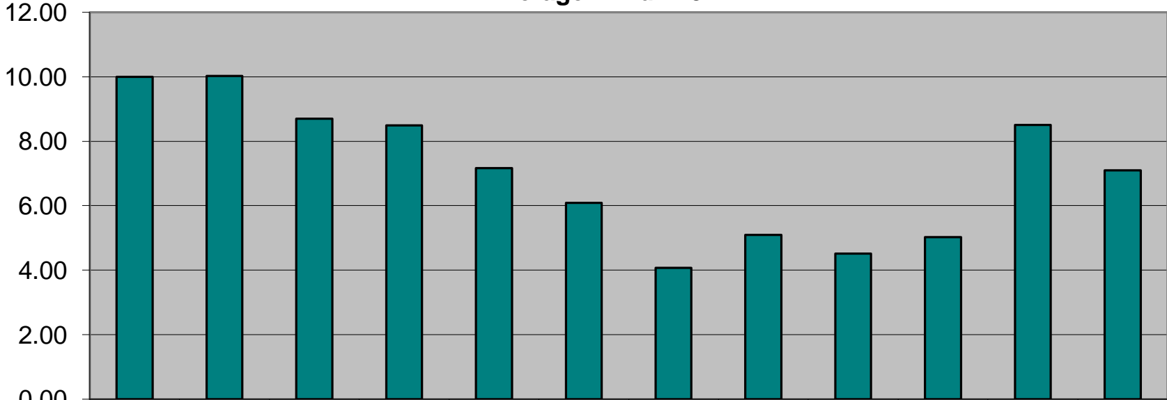
Average Wind - 1941
