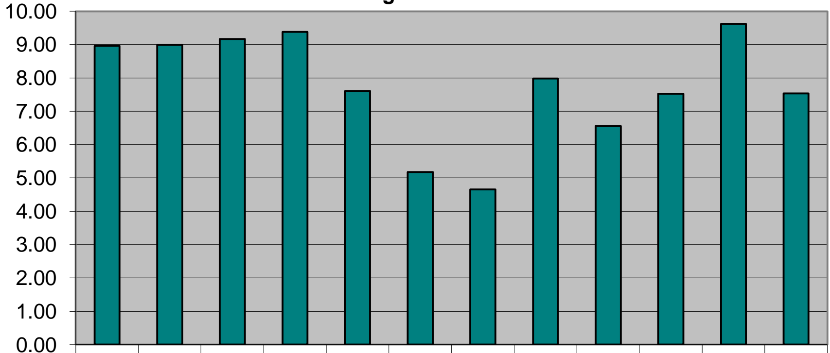
Average Wind - 1940
