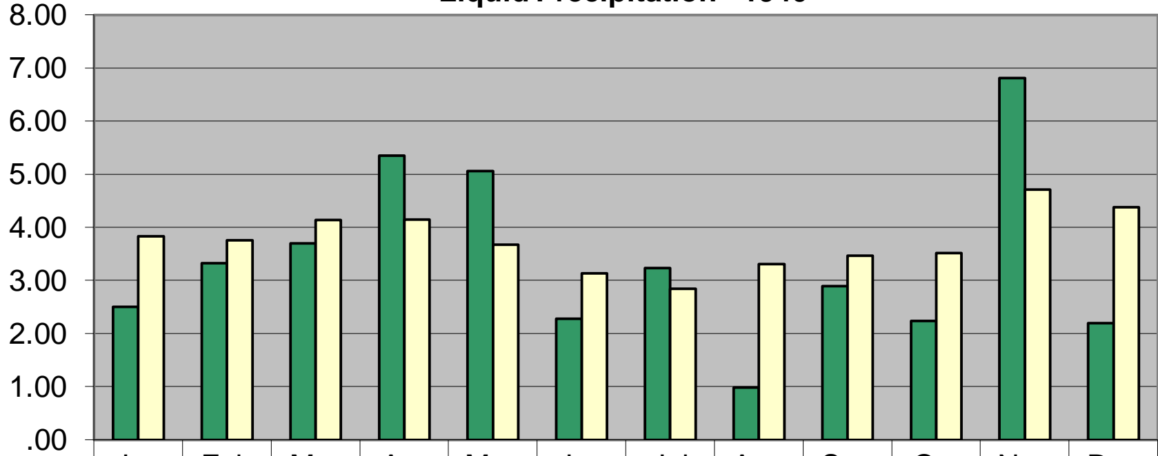
Liquid Precipitation - 1940
