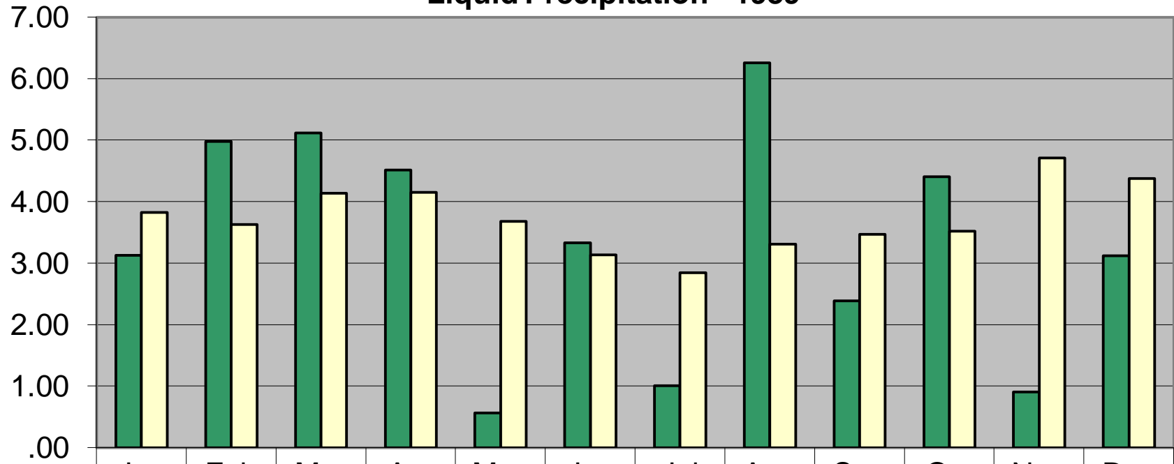
Liquid Precipitation - 1939
