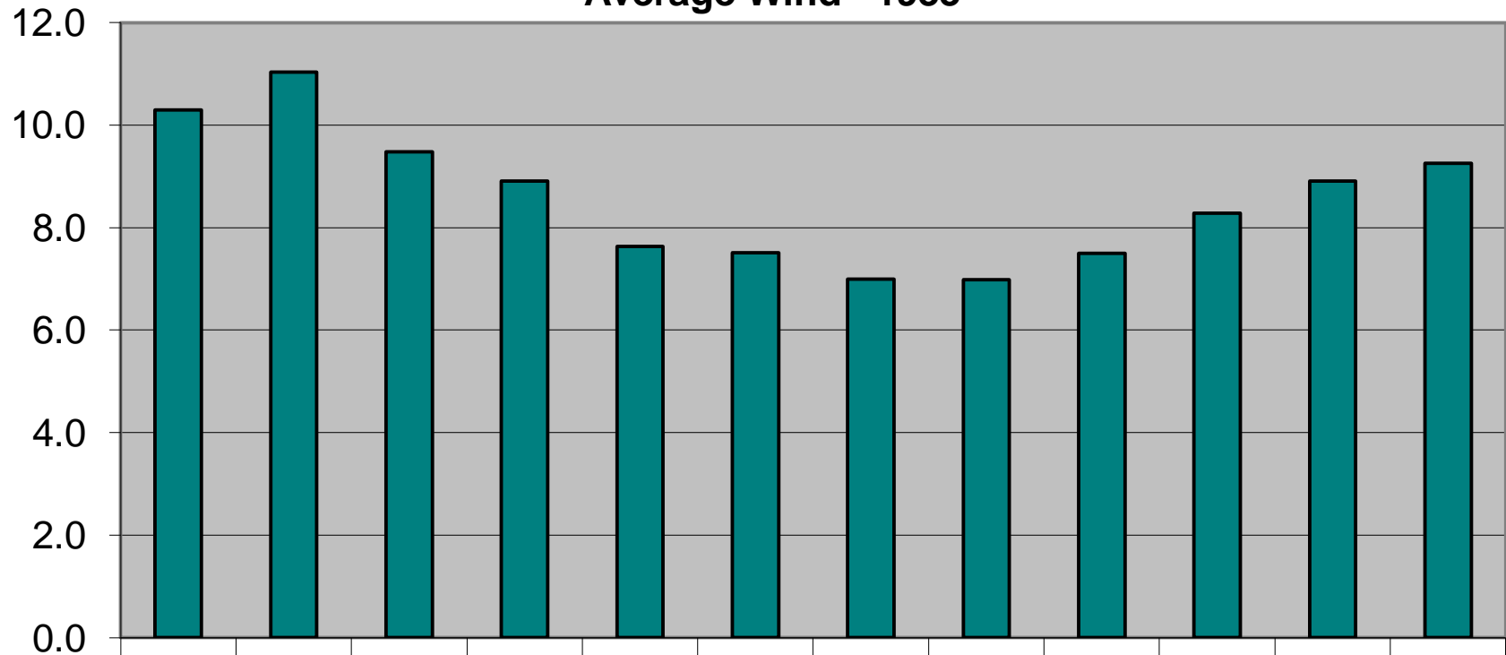
Average Wind - 1933
