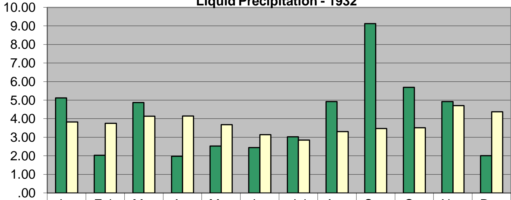
Liquid Precipitation - 1932
