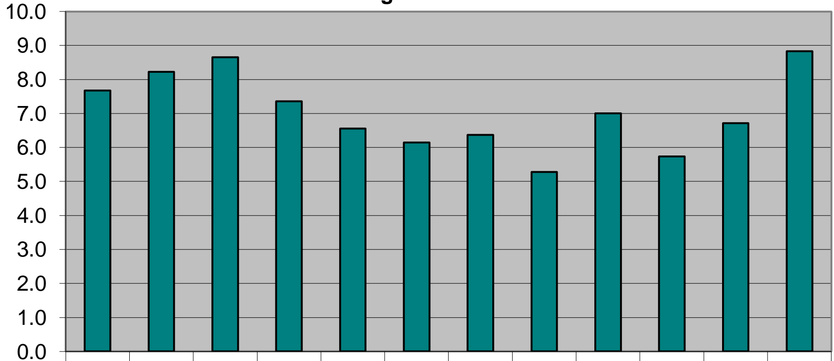
Average Wind - 1931
