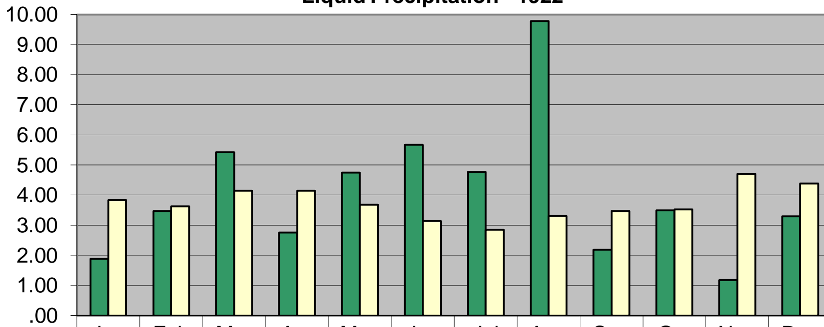
Liquid Precipitation - 1922
