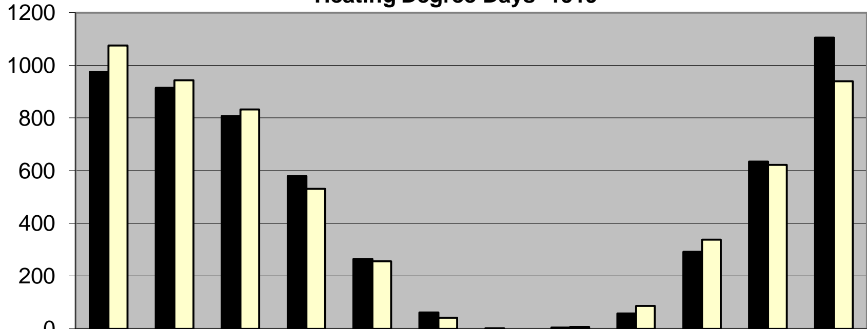
Heating Degree Days -1919
