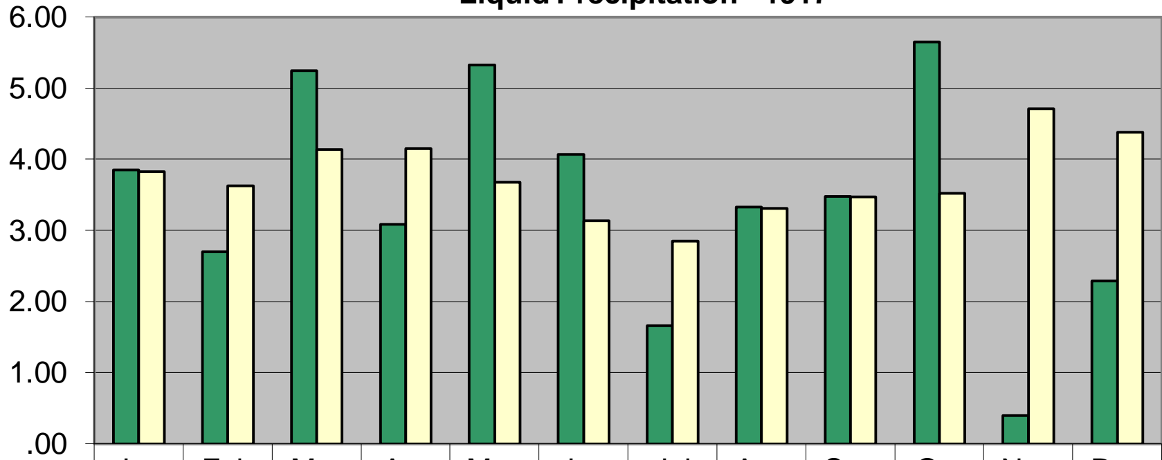
Liquid Precipitation - 1917
