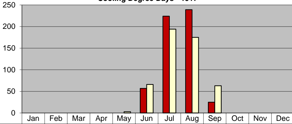
Cooling Degree Days - 1917
