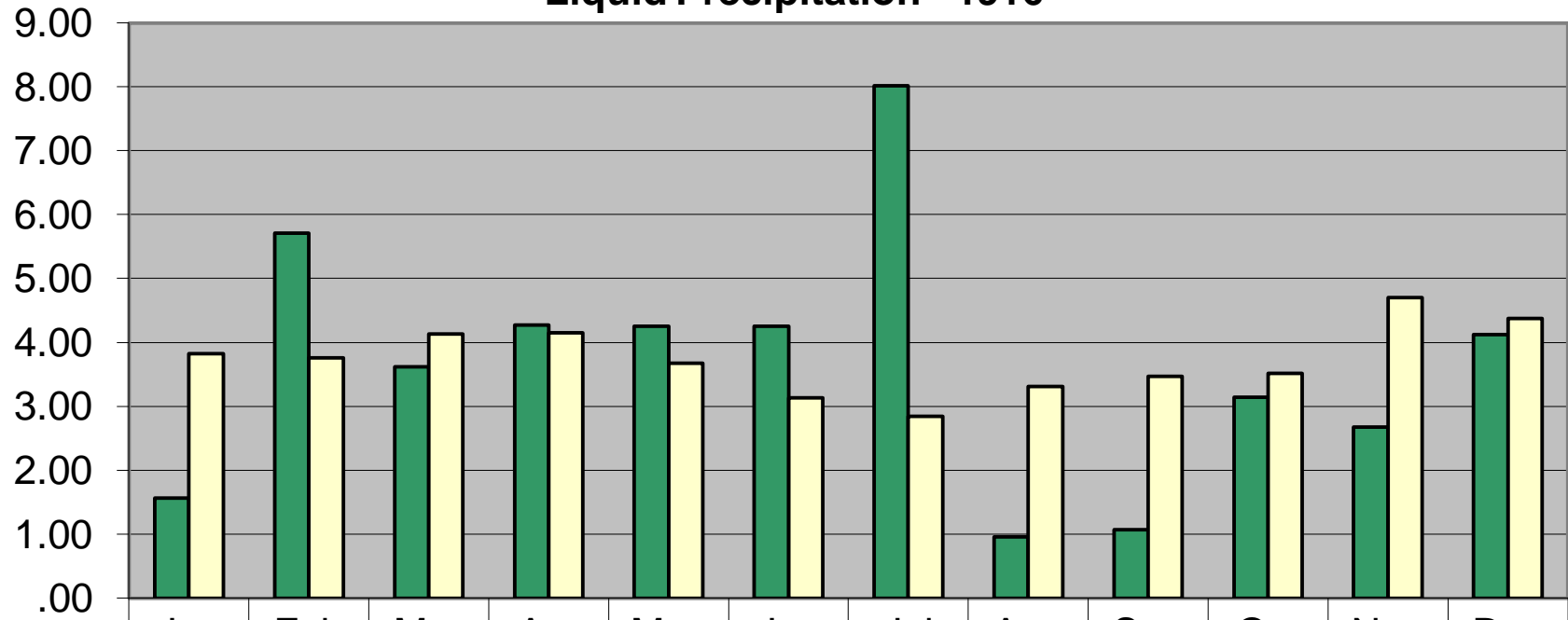
Liquid Precipitation - 1916
