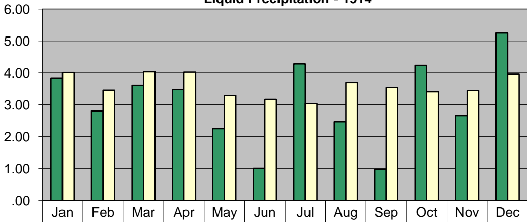
Liquid Precipitation - 1914
