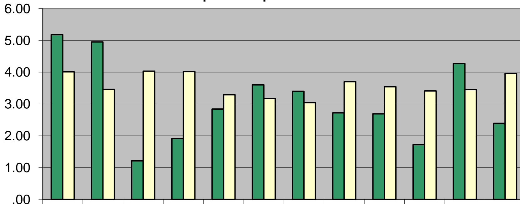
Liquid Precipitation - 1910
