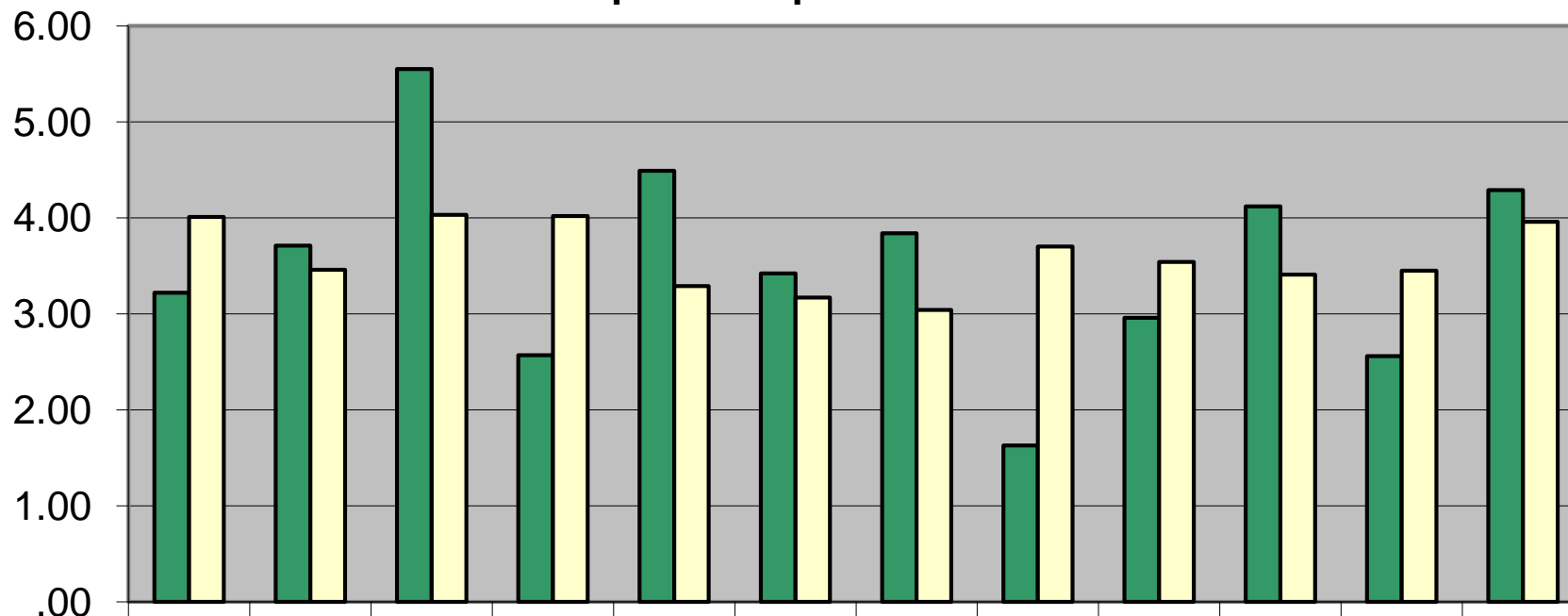
Liquid Precipitation - 1906
