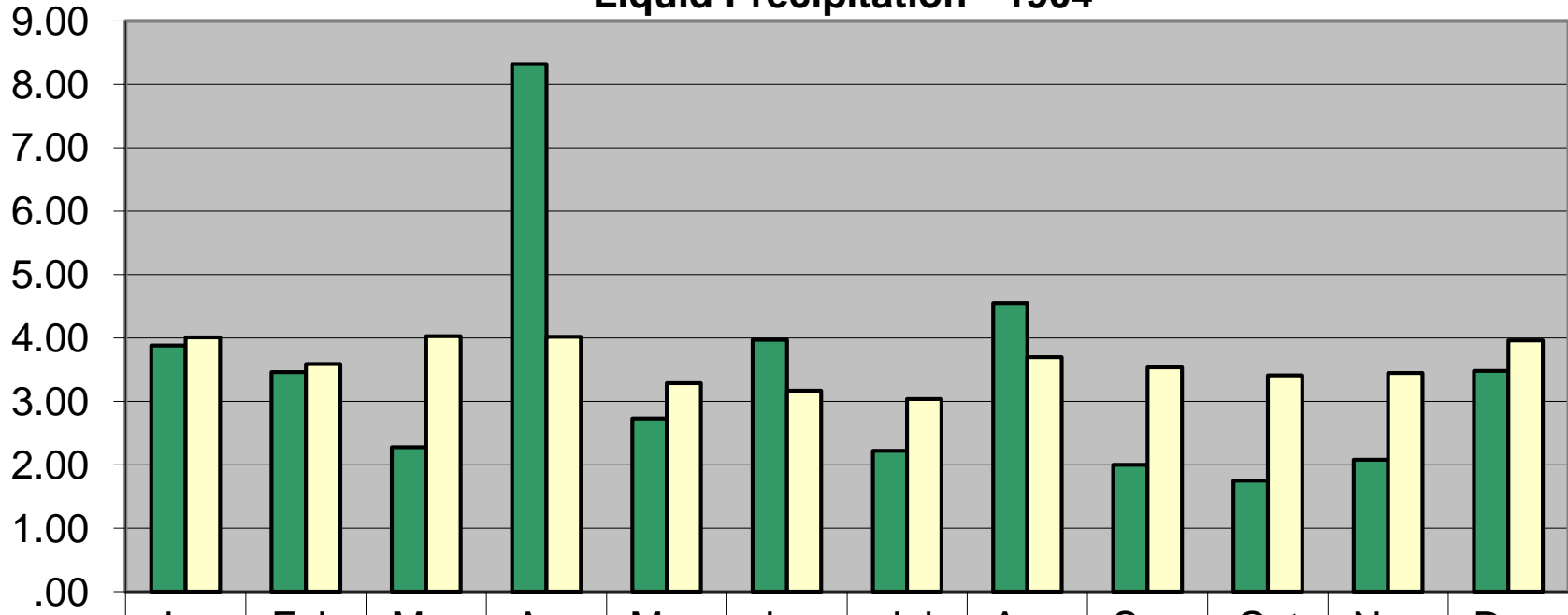
Liquid Precipitation - 1904
