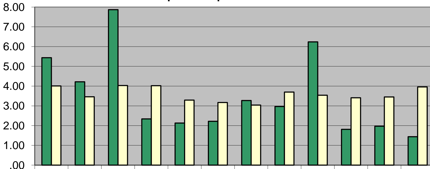
Liquid Precipitation - 1899
