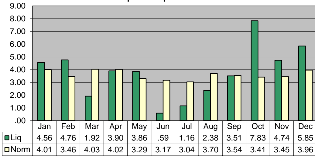
Liquid Precipitation - 1894
