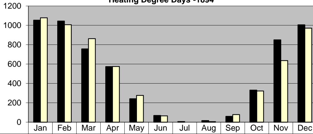
Heating Degree Days -1894
